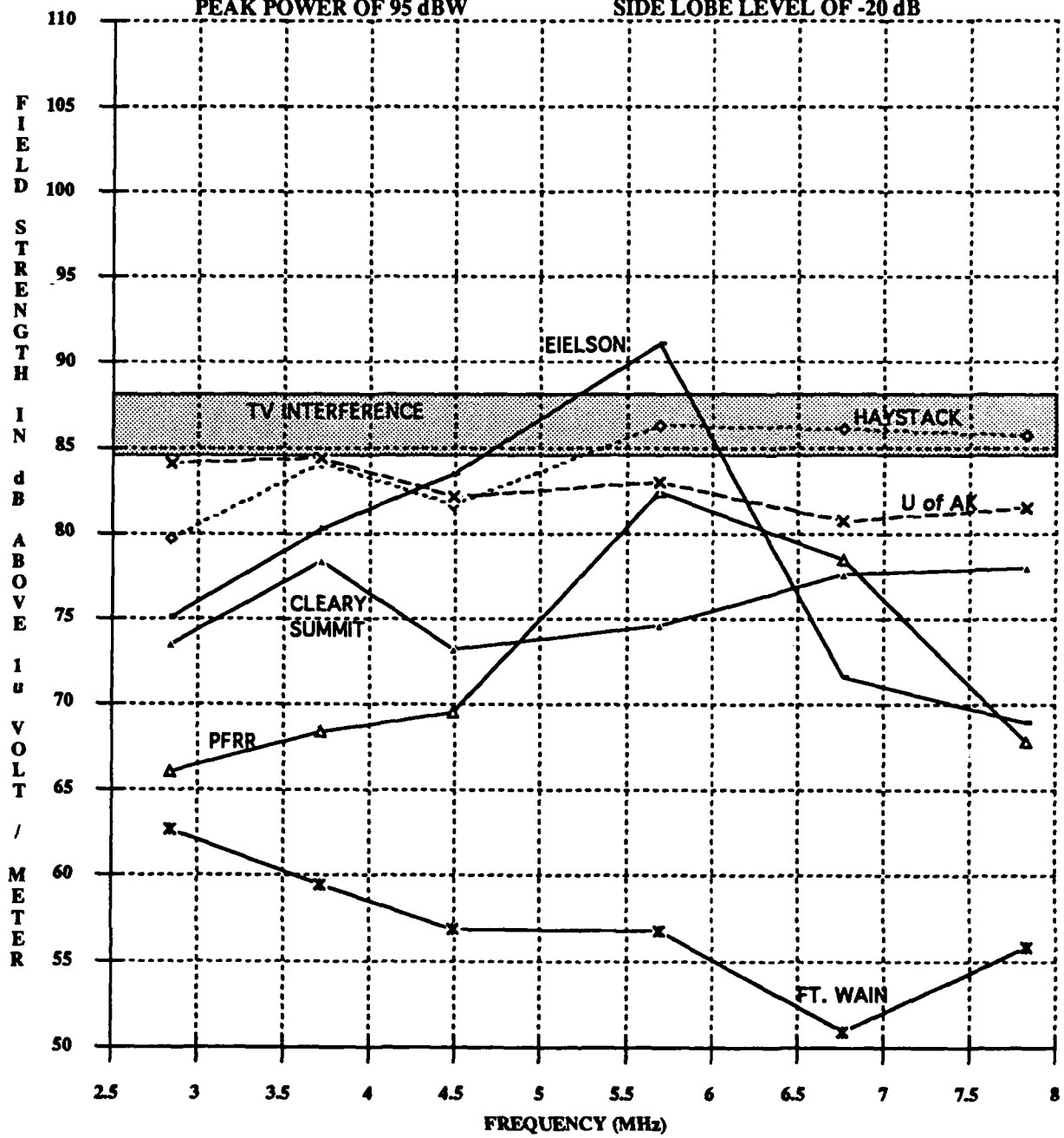
Figure 13. Phase II results with transmitter at Site # 12
