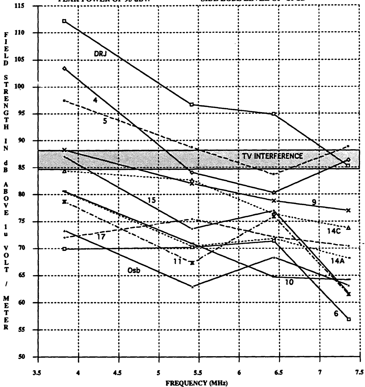
Figure 8. Phase I results with receiver at Poker Flat Research Range
