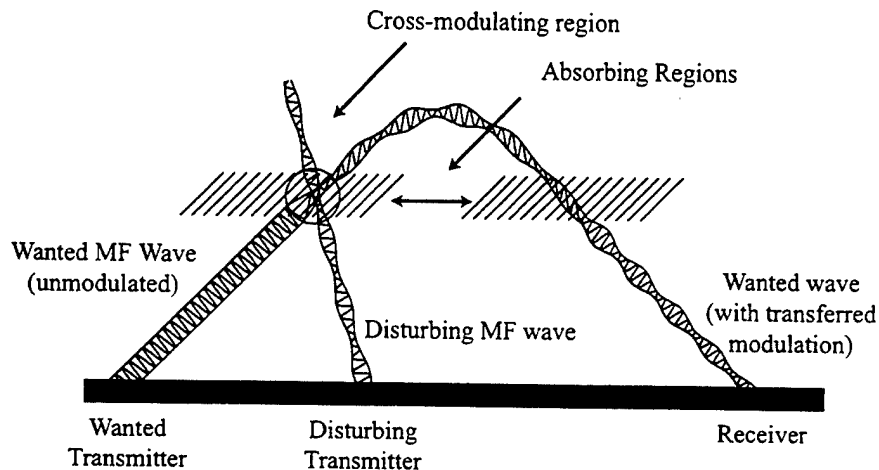
Figure 1.6: Geometry and nomenclature involved in ionospheric cross-modulation.
